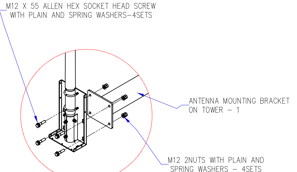
Omni directional antenna bracket Assembly Stage -4 Exploded View
