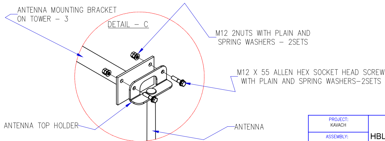
Omni directional antenna bracket Assembly Stage -5 Exploded View
