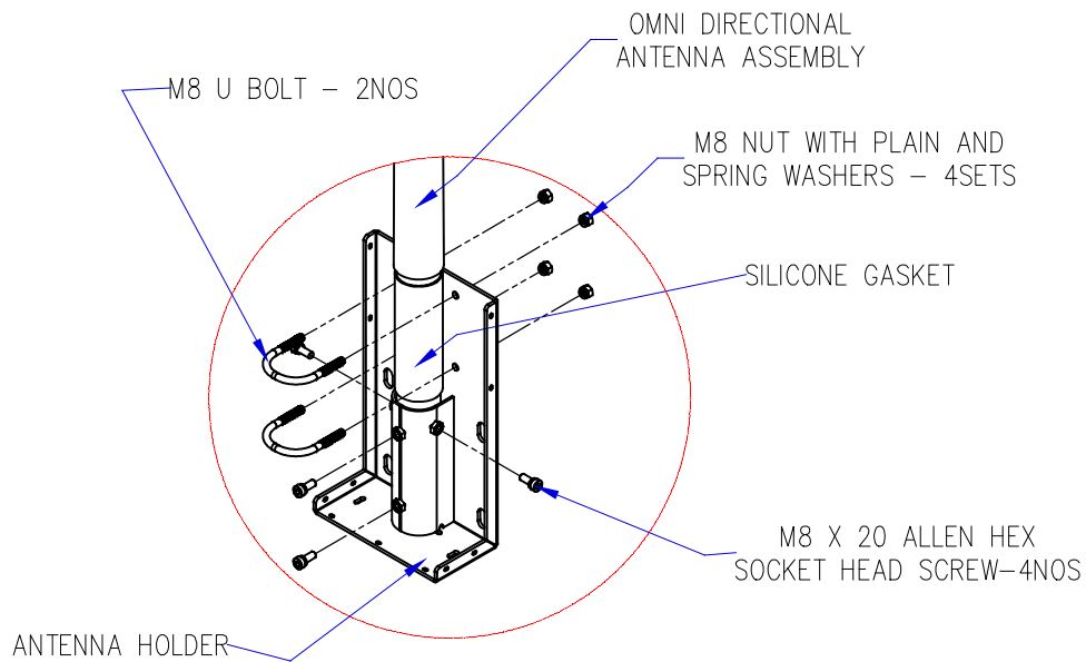
Omni directional antenna holder Assembly Stage -3 Exploded View
